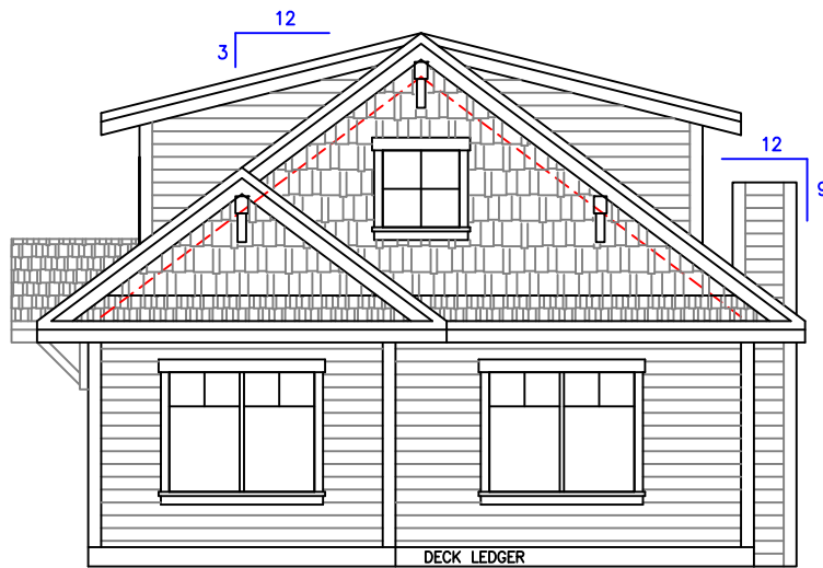
ELK RIDGE - POPLAR - FRONT ELEVATION
