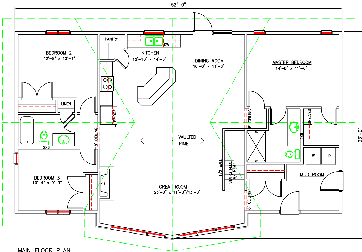
MAIN FLOOR PLAN AREA = 1580 sq. ft.
