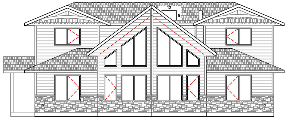
LOEHDORF FRONT ELEVATION
