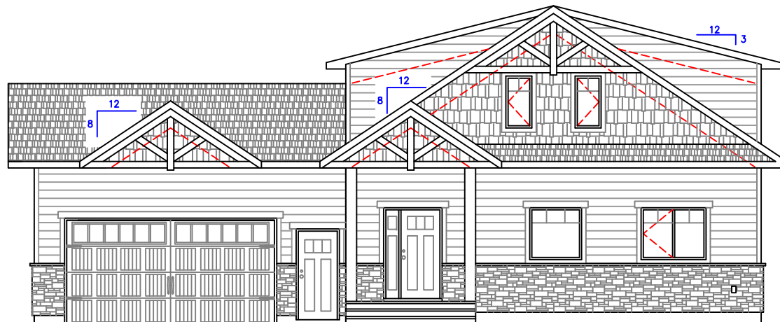
SASKATOON LOTTO 2017 FRONT ELEVATION
