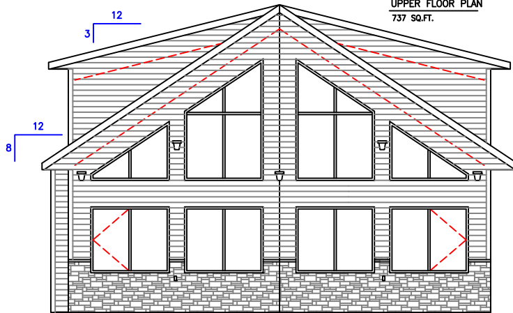
WILLIAMS FRONT ELEVATION
