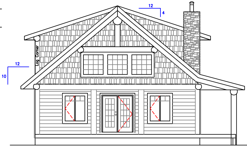
ZACHARIAS FRONT ELEVATION
