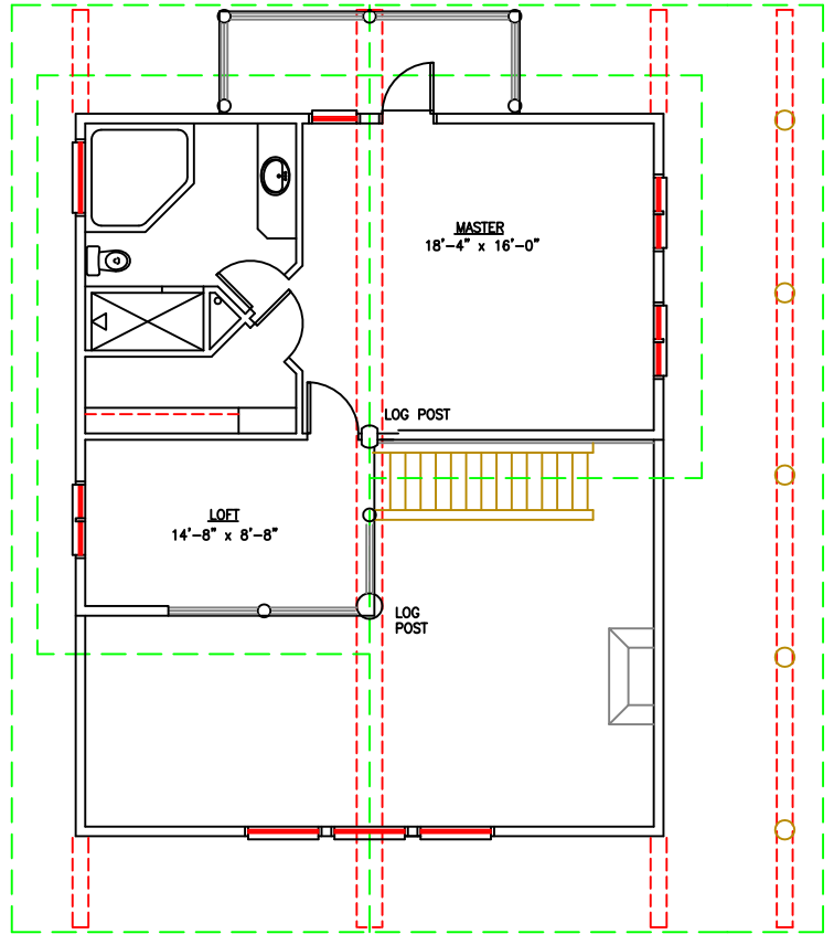
UPPER FLOOR PLAN 664 SQ.FT.
