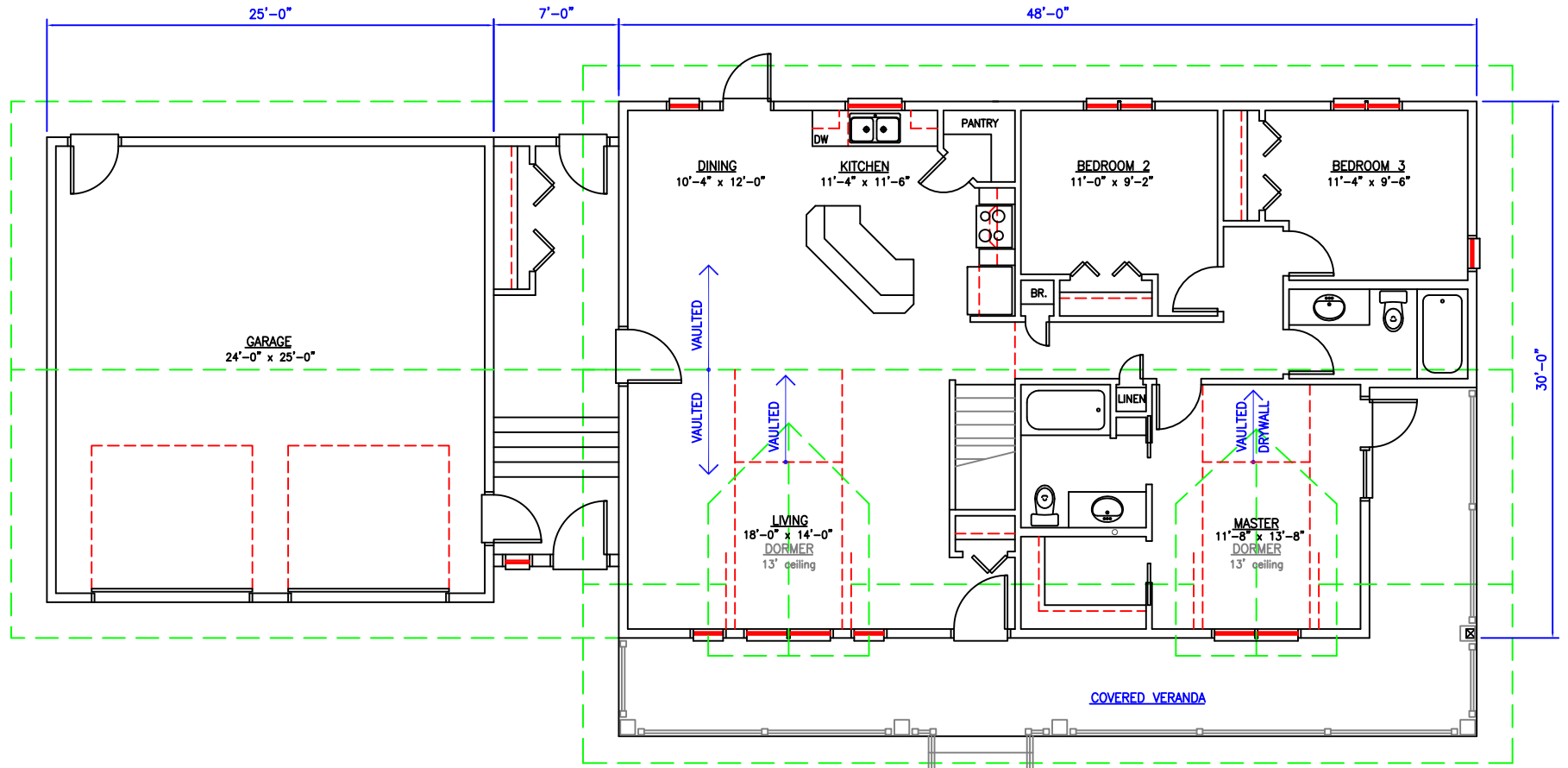
MAIN FLOOR PLAN Area = 1356 sq. ft.
