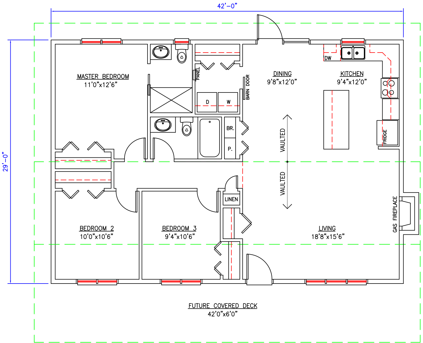
MAIN FLOOR PLAN 1227 sq. ft.
