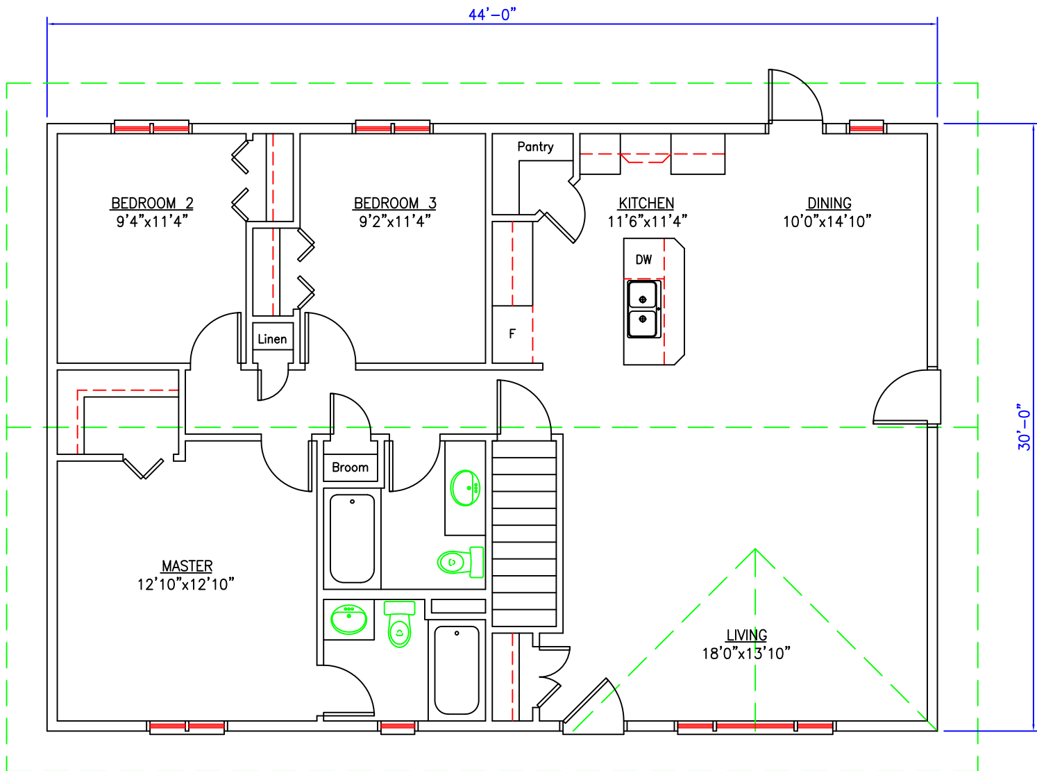
MAIN FLOOR PLAN 1320 sq. ft.
