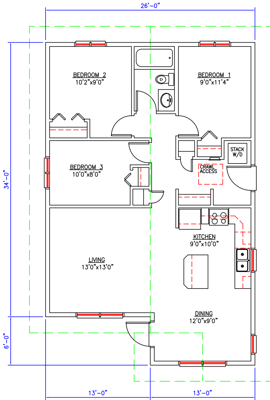
MAIN FLOOR PLAN 962 sq. ft.
