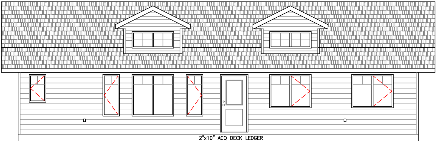
WATHAMAN FRONT ELEVATION
