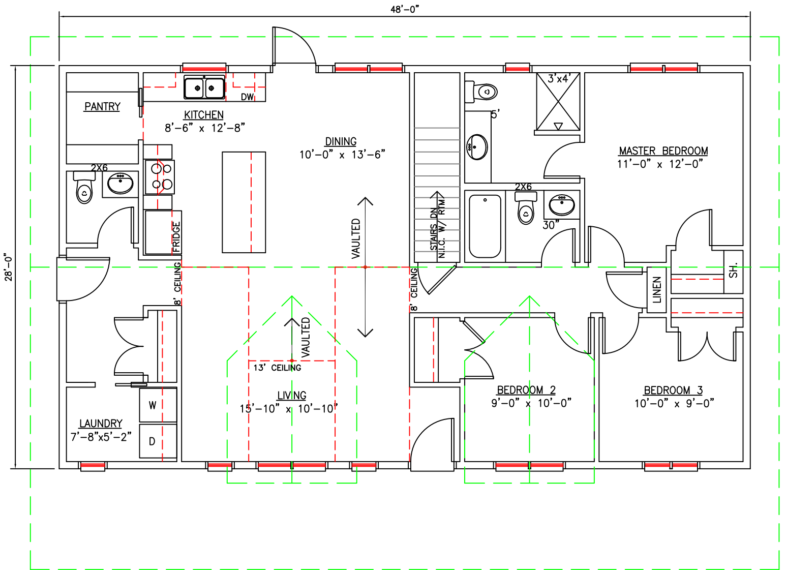
MAIN FLOOR PLAN 1344 SQ.FT.
