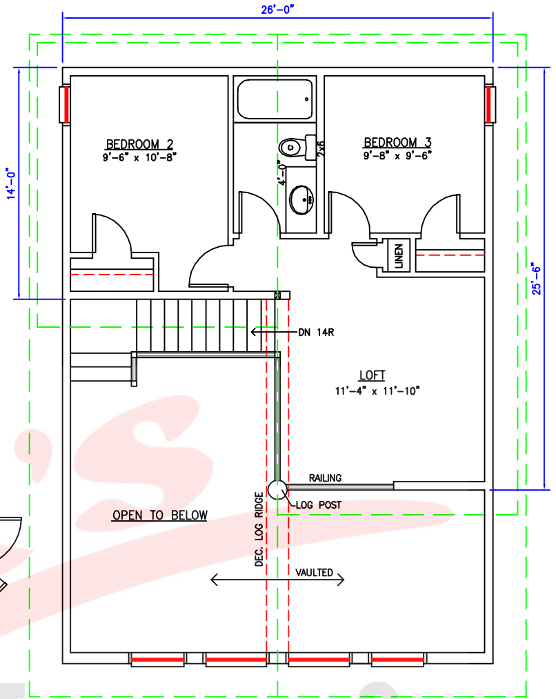
UPPER FLOOR PLAN 517 SQ.FT.
