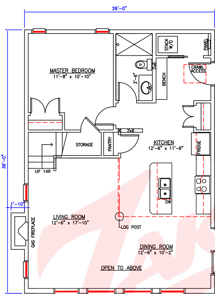
MAIN FLOOR PLAN 945 SQ.FT.
