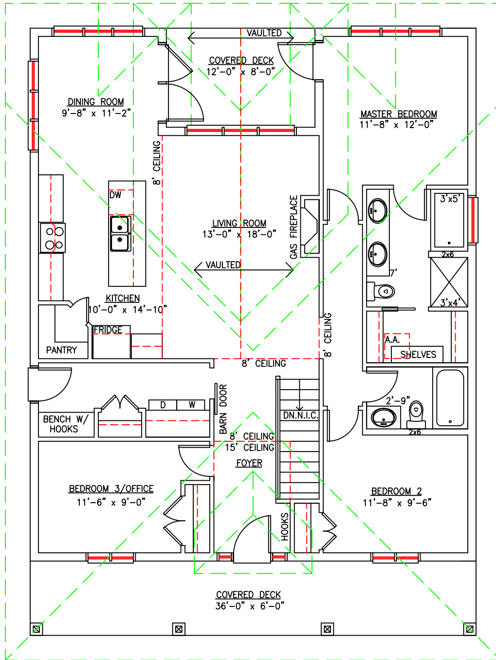
MAIN FLOOR PLAN 1452 SQ.FT.
