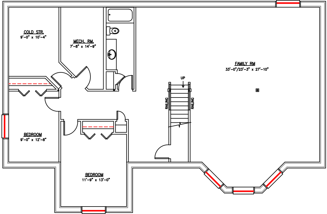
BASEMENT FLOOR PLAN 1652 SQ.FT
