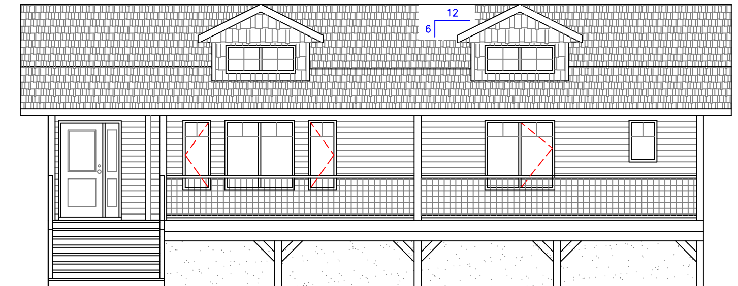
DYCK FRONT ELEVATION
