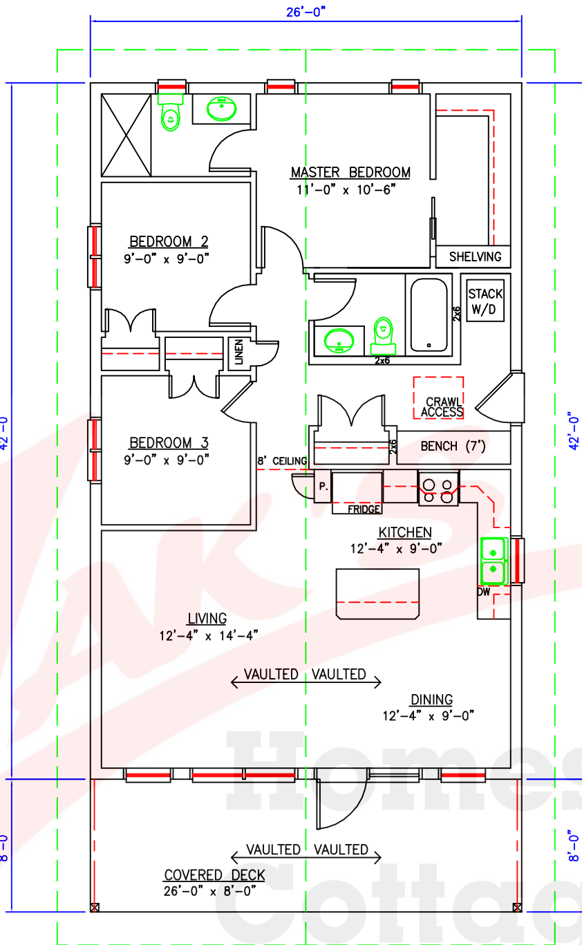
MAIN FLOOR PLAN 1092 SQ.FT.
