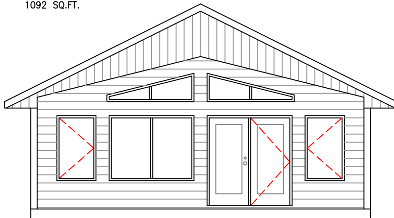
BOOTH FRONT ELEVATION
