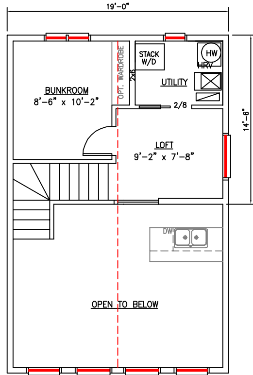
UPPER FLOOR 242 SQ.FT.
