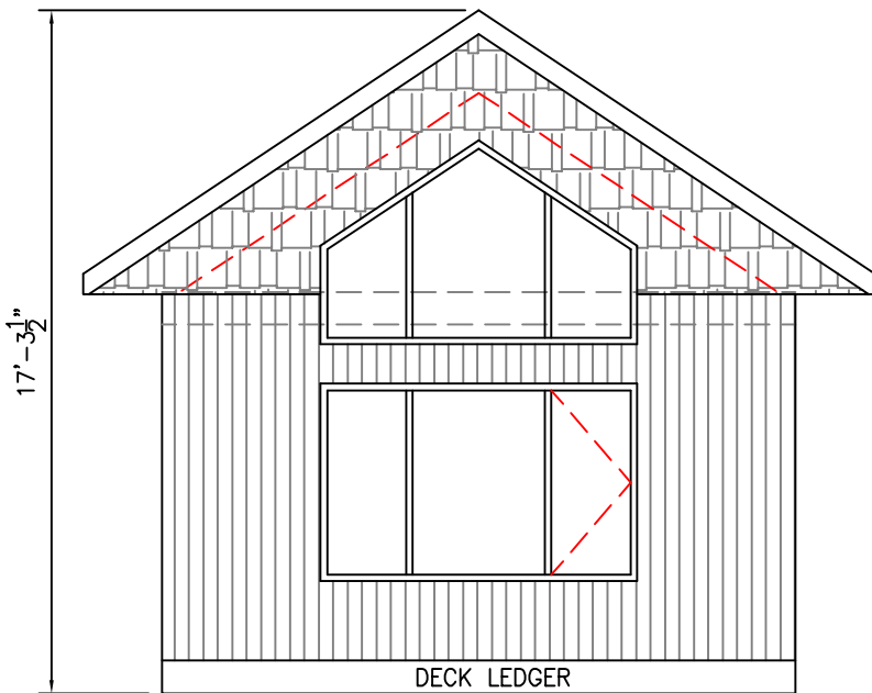
FRONT ELEVATION SCALE: 3/16"=1'-0"
