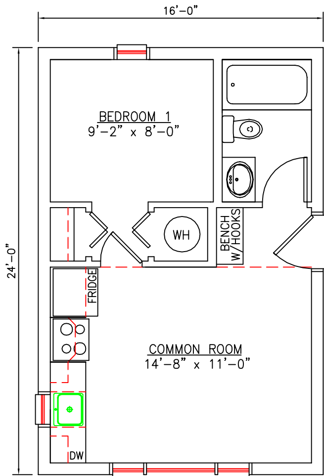
MAIN FLOOR PLAN 384 SQ.FT.
