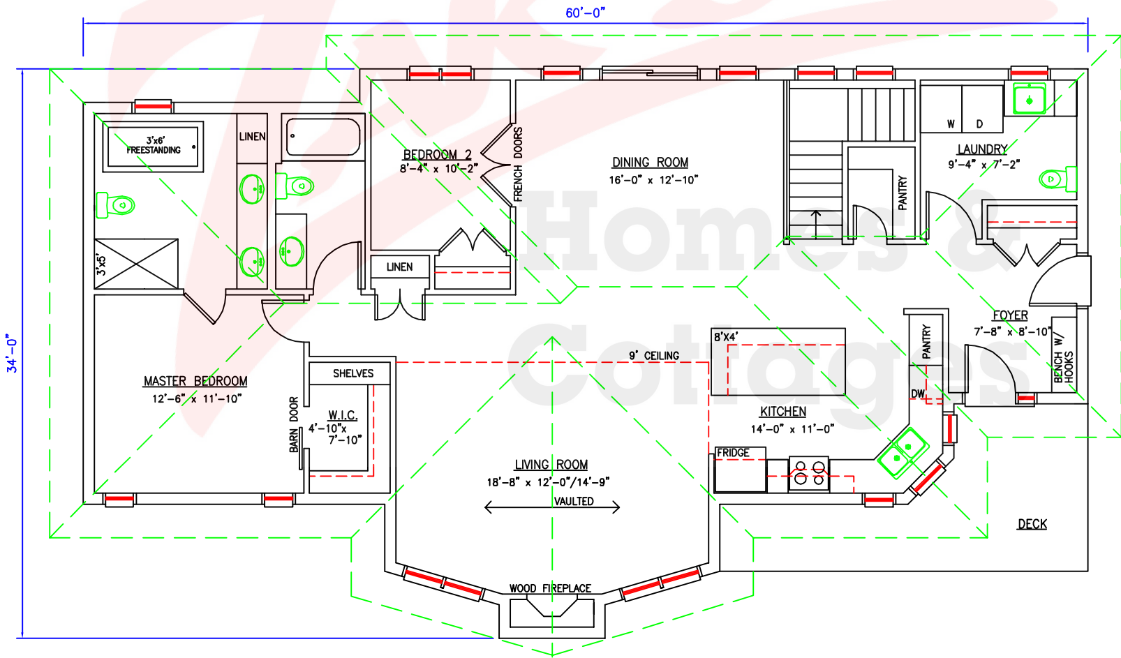
MAIN FLOOR PLAN 1594 SQ.FT.
