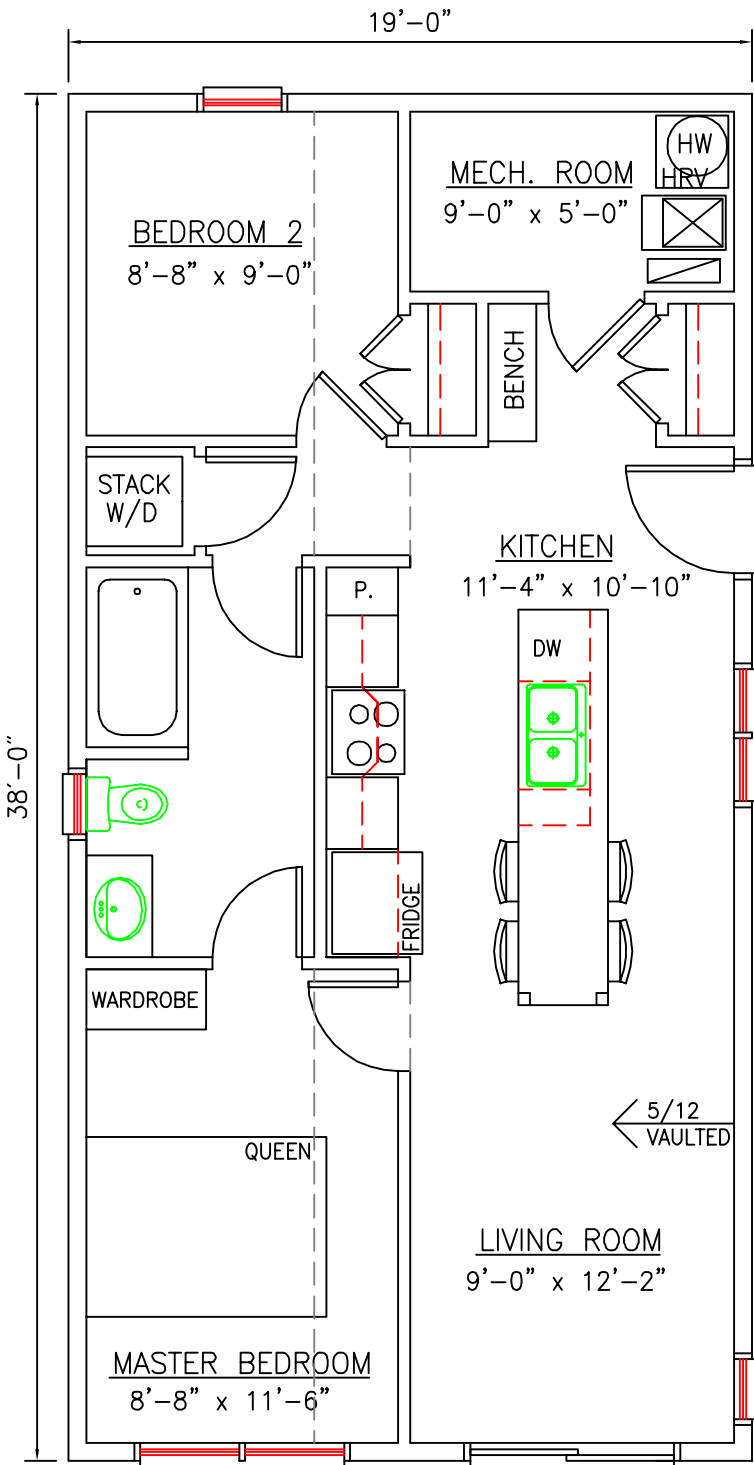
MAIN FLOOR PLAN 722 SQ.FT.
