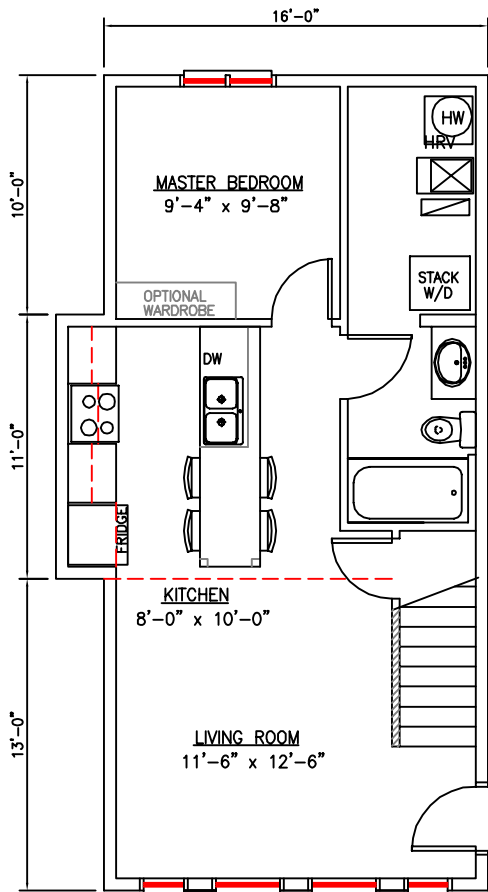
MAIN FLOOR 566 SQ.FT. TOTAL 888 SQ.FT.
