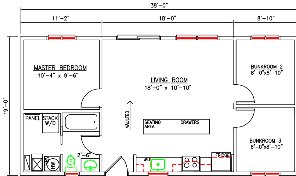
MAIN FLOOR PLAN 722 SQ.FT. SCALE: 1/8"=1'-0"
