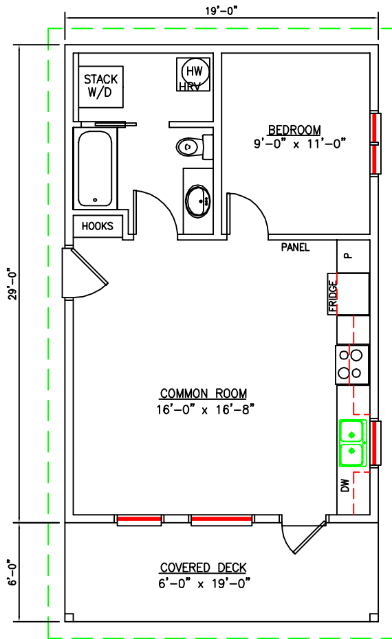
MAIN FLOOR PLAN 551 SQ.FT.
