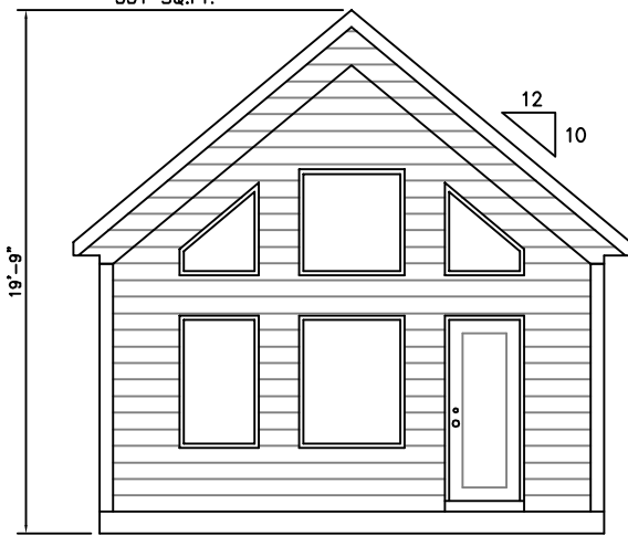
FRONT ELEVATION
