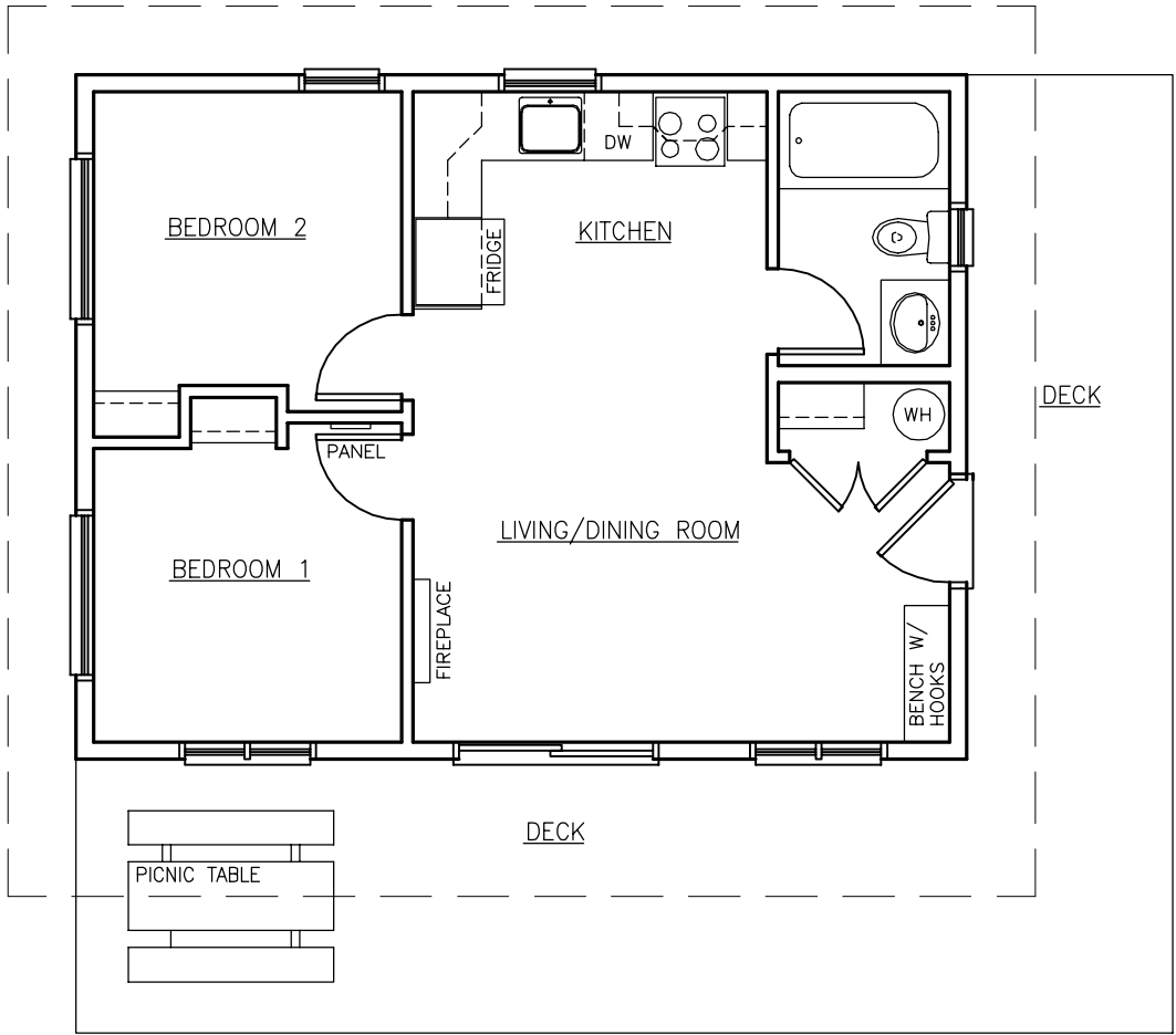
MAIN FLOOR PLAN 520 SQ.FT
