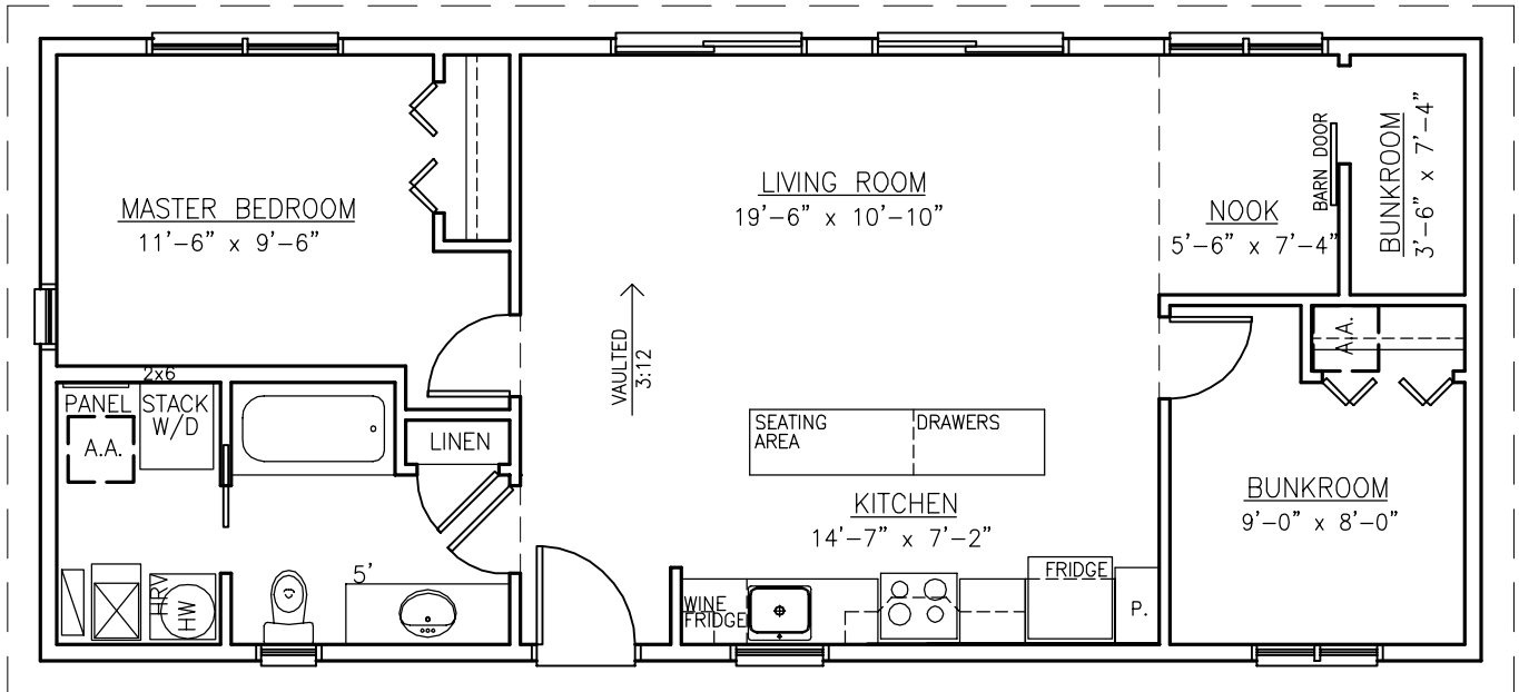
MAIN FLOOR PLAN 836 SQ.FT.
