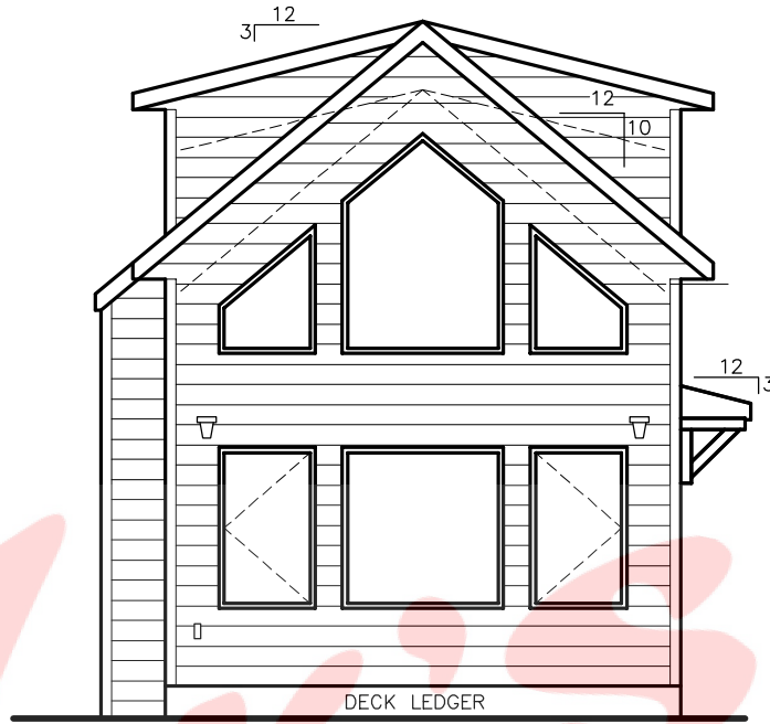
SERENITY FRONT ELEVATION
