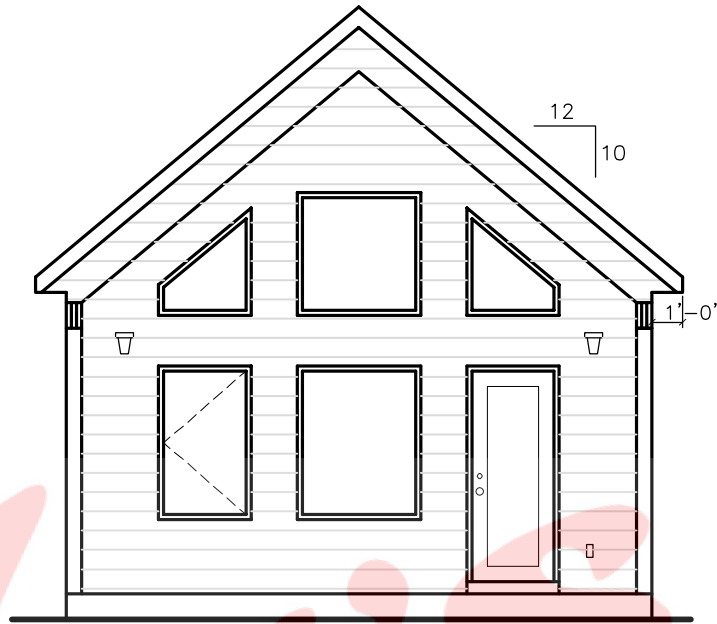
FRONT ELEVATION
