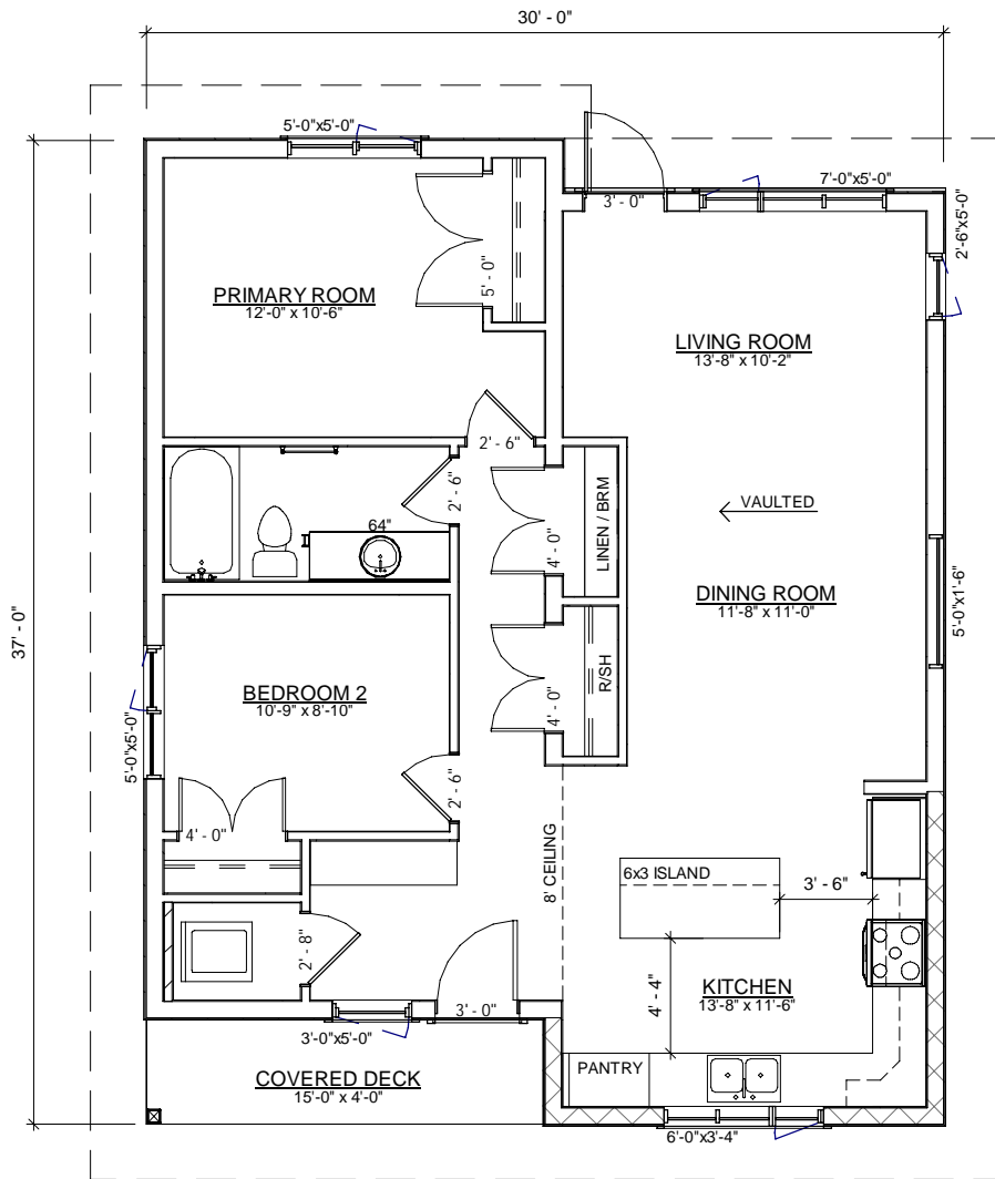
MAIN FLOOR PLAN SCALE 1/8" = 1'-0" 1020 SQFT
