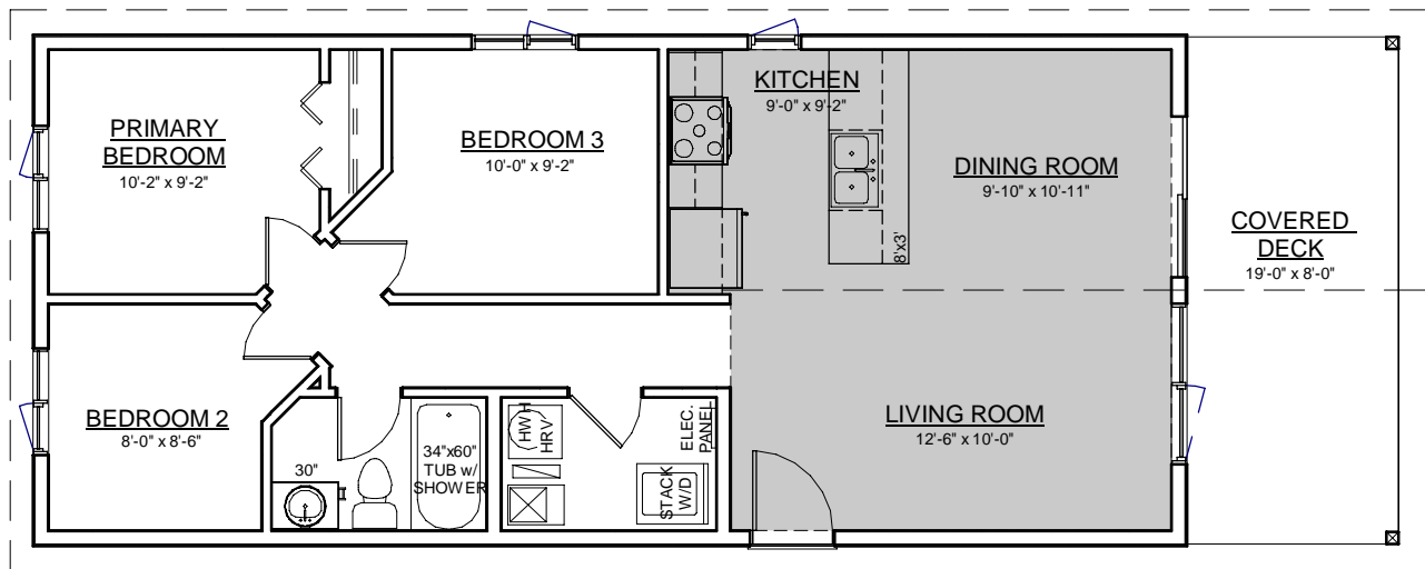
MAIN FLOOR PLAN SCALE 1/8" = 1'-0" 817 SQFT
