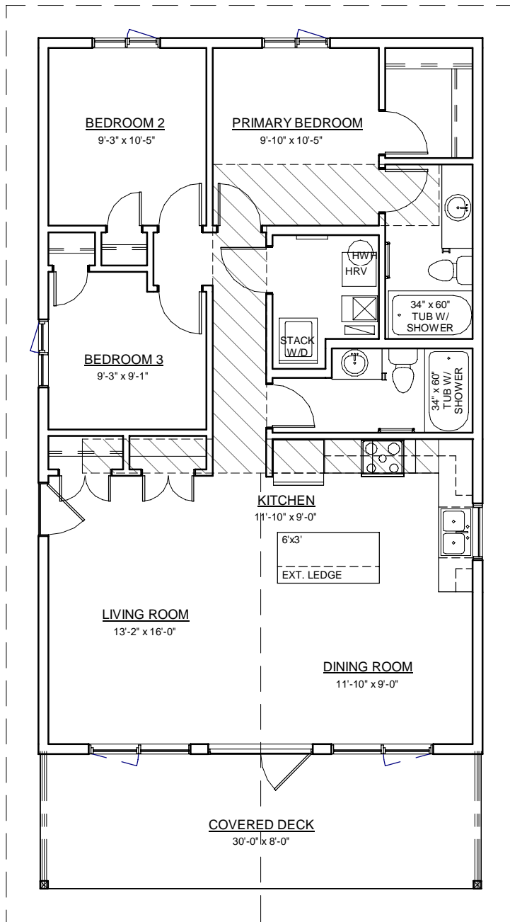
MAIN FLOOR PLAN SCALE 1/8" = 1'-0" 1092 SQFT
