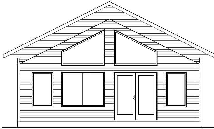
SMOOTHSTONE FRONT ELEVATION
